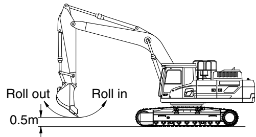
Bucket cylinder
