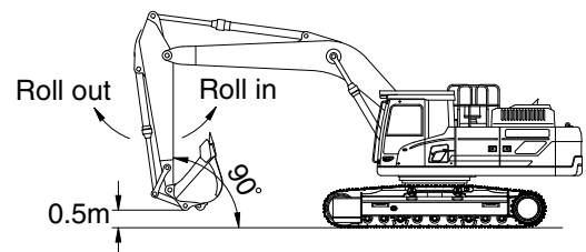
Arm cylinder
